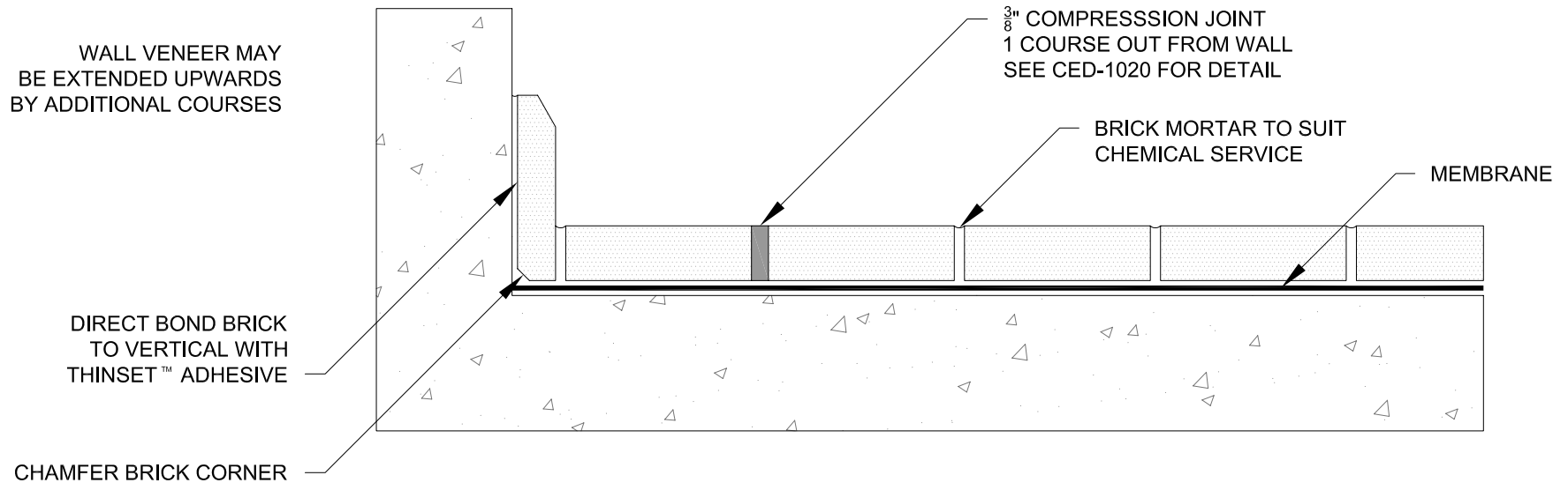
SECTION VIEW ABOVE TYPIFIES BRICK / MEMBRANE CONSTRUCTION SECTION VIEW BELOW TYPIFIES DIRECT BOND CONSTRUCTION
